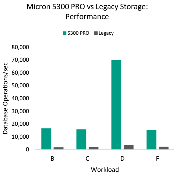
Figure 3: Performance
