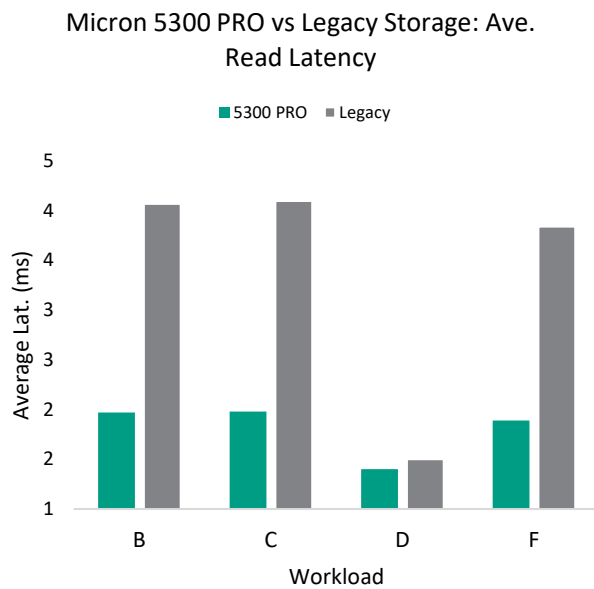
Figure 4: Latency
