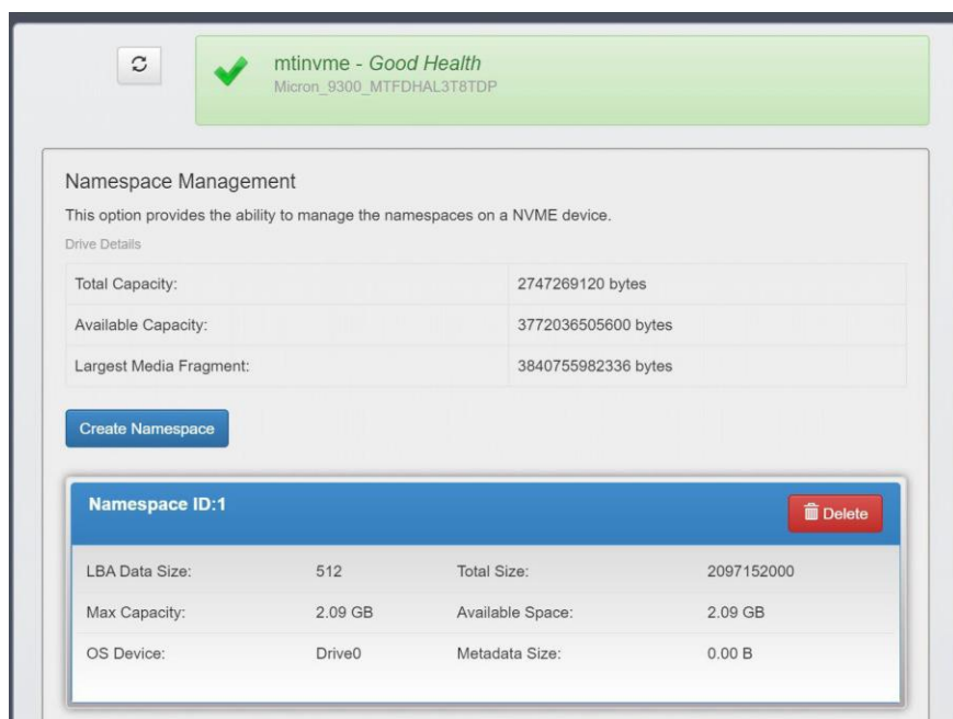
Figure 24: Namespace Management
