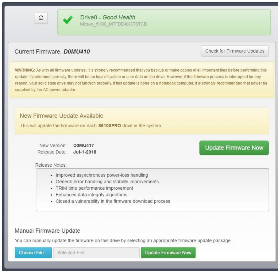
Figure 13: Update Firmware
