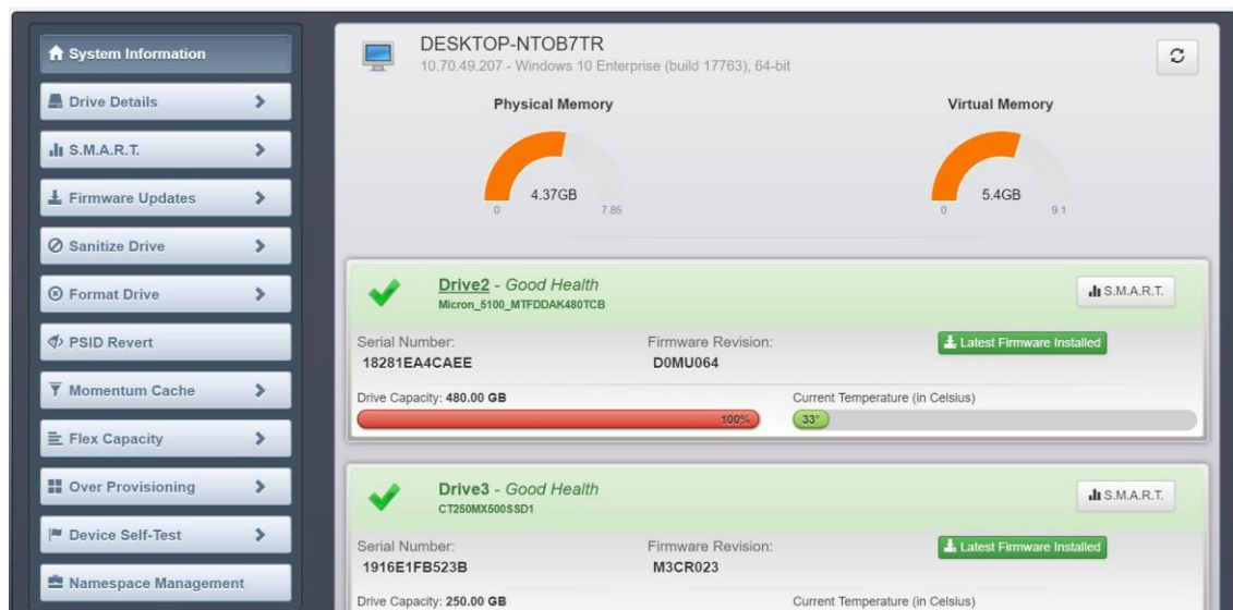
Figure 1: System Information
