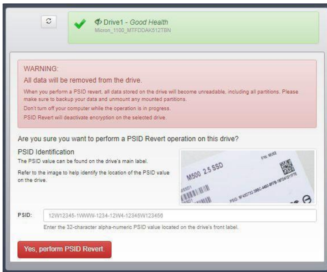
Figure 19: PSID Revert
