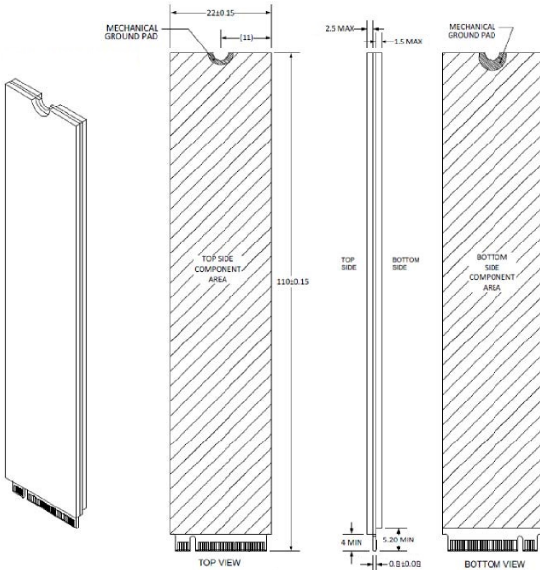
Figure 4: Nominal Dimensions
