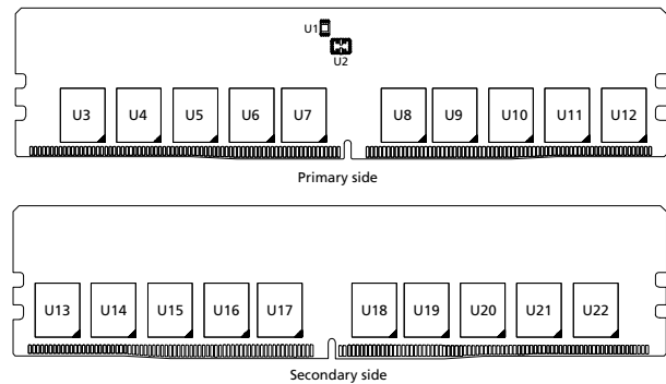
Figure 1: 288-Pin DDR5 EUDIMM (R/C-E0)
