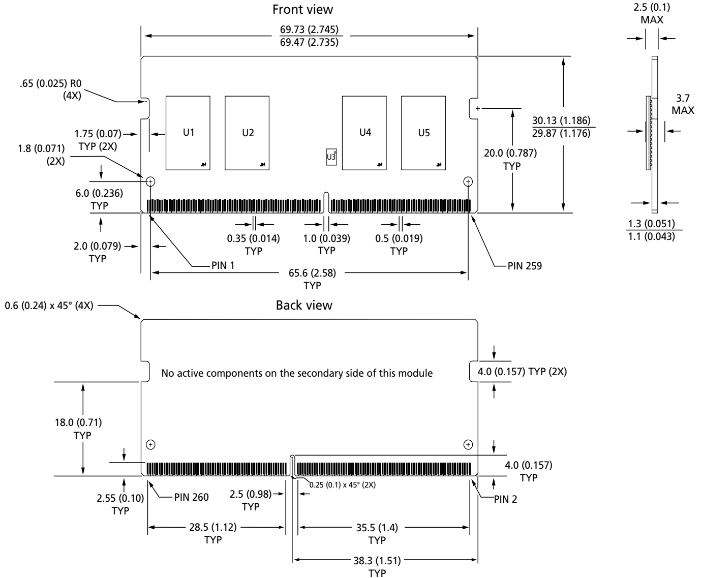
Figure 2: 260-Pin DDR4 SODIMM
